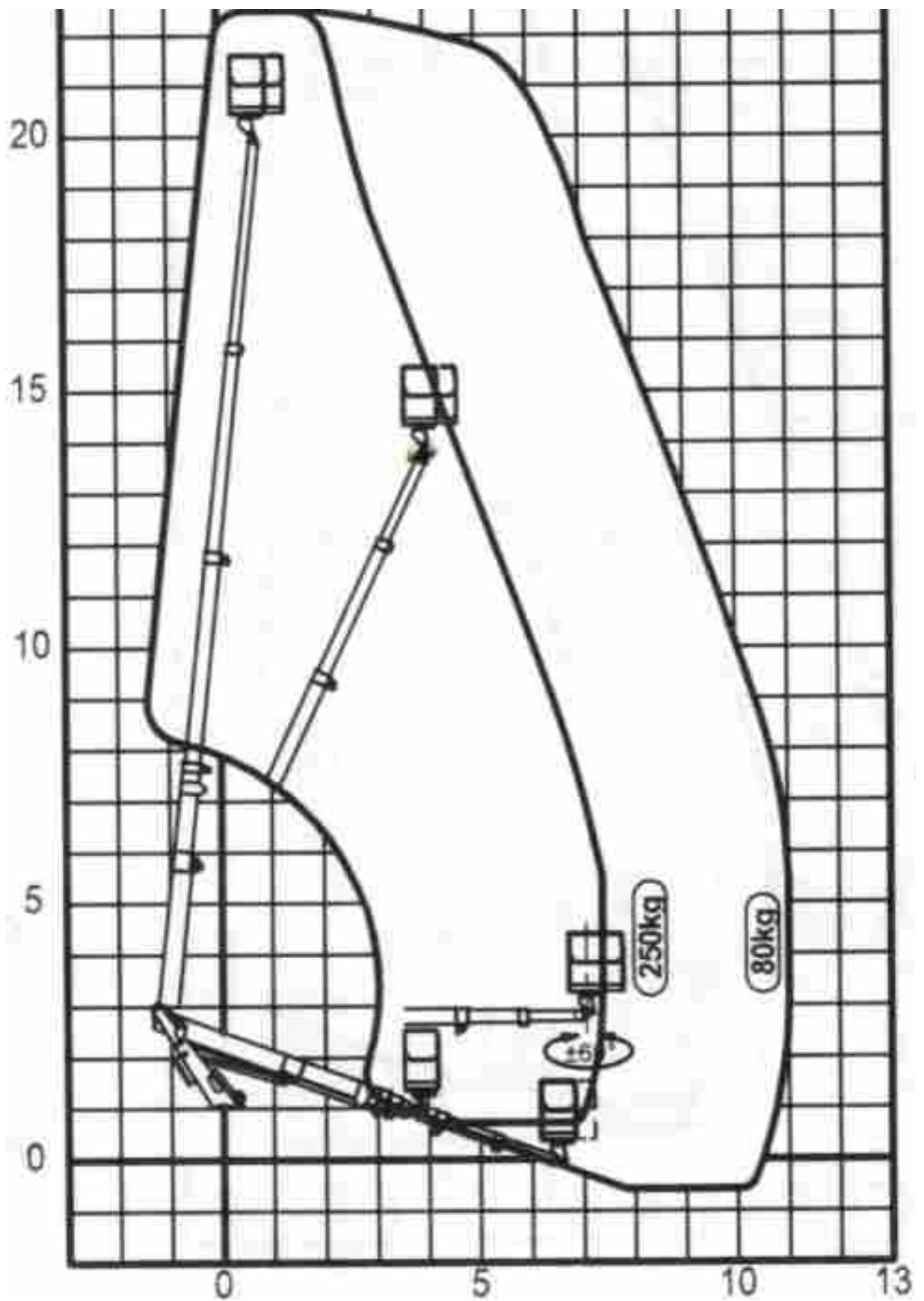
Palfinger P480
